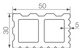
joist dimensions (mm)
