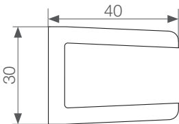
Channel section
