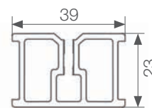
aluminum joist dimensions (mm)
